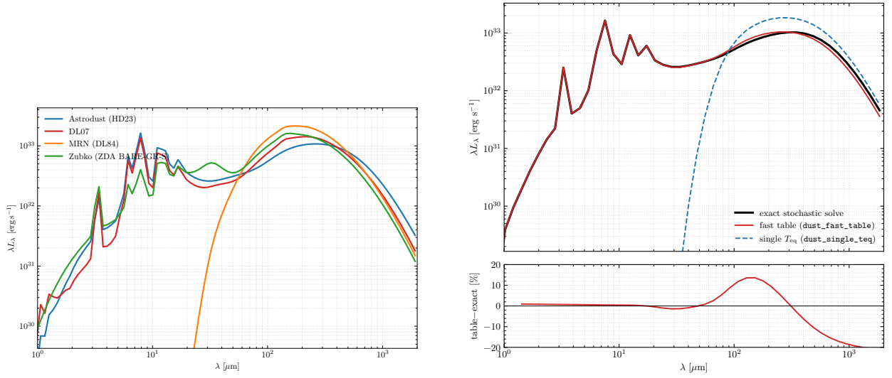
Figure 2: Left : the emission spectrum of a single cell heated by the same radiation field, for the four SEDUST grain models (astrodust, dl07, mrn, zubko); the total power is identical (each is normalized to the absorbed luminosity) while the PAH bands and the far-infrared slope differ by model. Right : the par%dust_fast_table approximation against the exact stochastic solve — the total luminosity is identical, the PAH/mid-infrared region agrees to \sim 1\% , and the largest deviations sit on the far-infrared slope.
