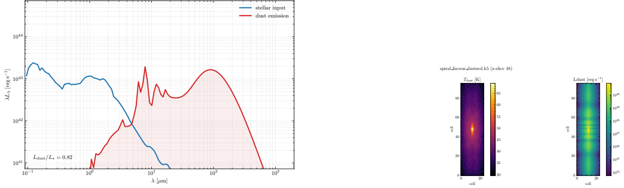
Figure 1: Left : the UV-to-FIR SED of the examples/galaxy model (exponential disk + Sersic bulge): the attenuated starlight and the thermal dust emission (PAH bands and a far-infrared peak), with L_{\text{dust}}/L_{\star} \approx 0.8 . Right : the mid-plane dust-emission luminosity of the spiral_faceon.in model, showing the m = 2 log-spiral arms imposed on the dust density.
