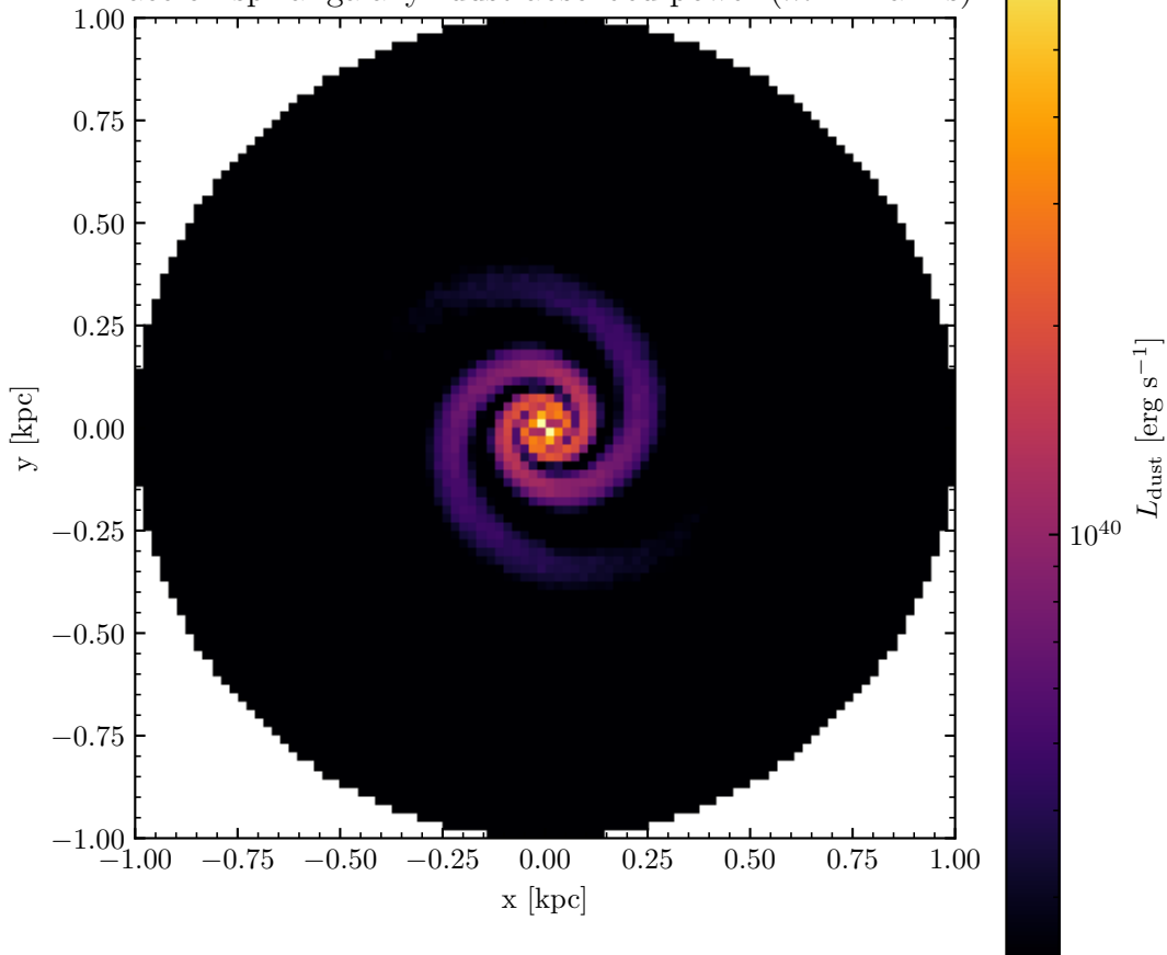
face-on spiral galaxy: dust absorbed power ( m = 2 arms)
