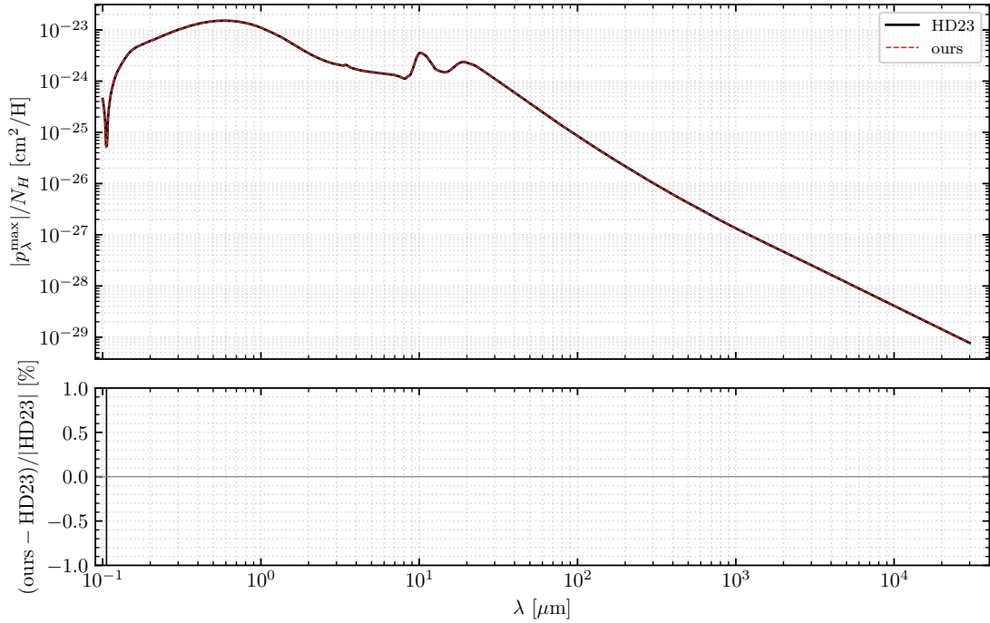
Figure 8: Top: |p_\lambda^{\max}|/N_H from HD23 polarized_extinction.dat (black solid) and from eq. 13 evaluated on the HD23 release Q tables (red dashed). Bottom: relative residual in percent. Peak value agrees to four significant figures.
