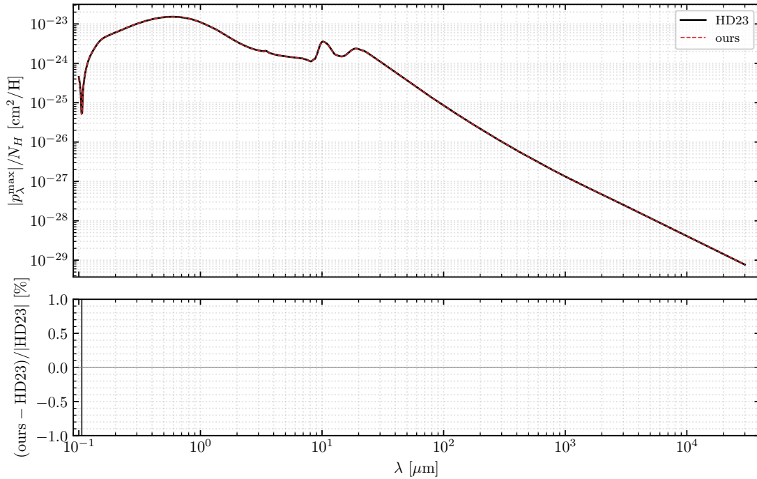
Figure 8: Top: |p_{\lambda}^{\text{max}}|/N_H from HD23 polarized_extinction.dat (black solid) and from eq. 13 evaluated on the HD23 release Q tables (red dashed). Bottom: relative residual in percent. Peak value agrees to four significant figures.
