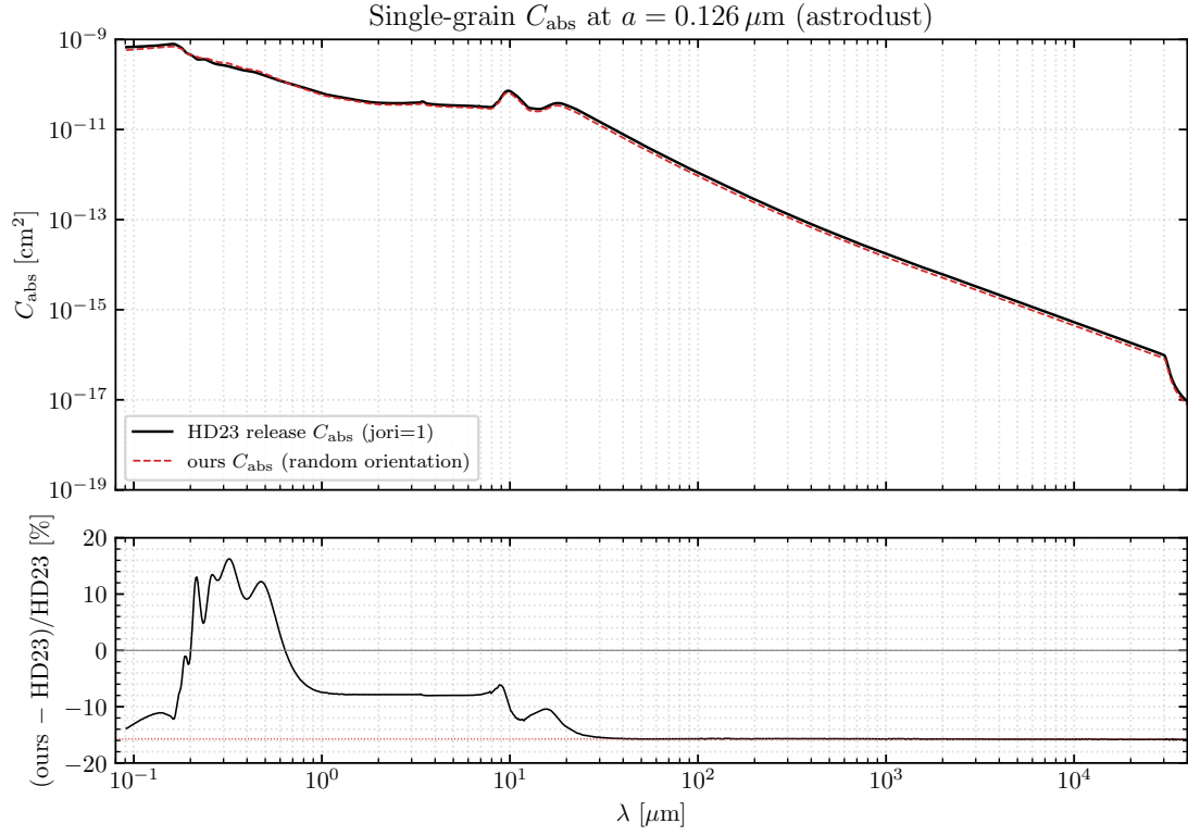
Figure 5: Single-grain absorption cross section at a = 0.126 \mu\text{m} . Top: HD23 release C_{\text{abs}} from \text{jori}=1 ( k\parallel a , black solid) and our C_{\text{abs}} from the random-orientation Q table that sed_init loads (red dashed); both tables share the DH21 wavelength grid, so no interpolation is involved. Bottom: relative residual (\text{ours} - \text{HD23})/\text{HD23} in percent. The flat -15.7\% plateau across 30 \mu\text{m} – 30000 \mu\text{m} is precisely the ratio (\frac{1}{3}Q_{\parallel} + \frac{2}{3}Q_{\perp})/Q_{\perp} for an oblate b/a = 1.4 spheroid in the dipole limit at this grain.
