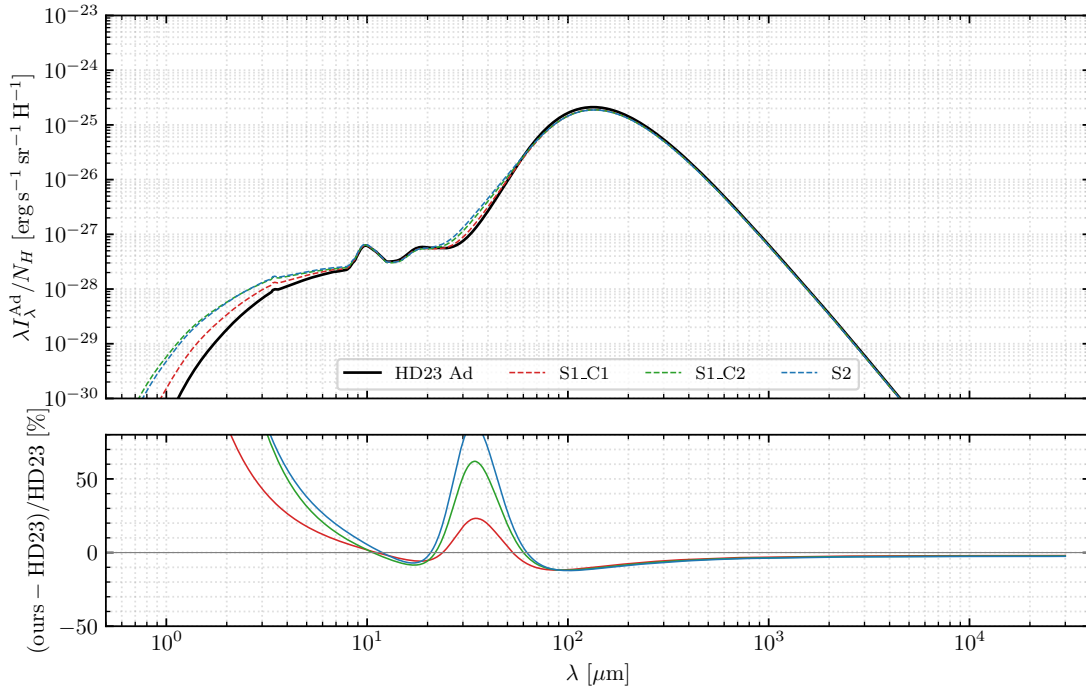
Figure 4: Astrodrust thermal emission per H atom at HD23 best-fit heating ( U = 1.585 ) for the current production (corrected Mathis 4000 K dilution, see §7.1.1). Top: our three enthalpy stages (S1_C1, S1_C2, S2) overlaid on HD23 astrodrust_irem.dat. Bottom: relative residual in percent. The FIR peak shape is recovered; a 10.1% systematic under-prediction persists at the 133 \mu\text{m} peak (down from 18.2% before the Mathis correction), and the < 5 \mu\text{m} range over-predicts by a few-times factor (a PAH-deficit issue; see Sect. 7.2).
