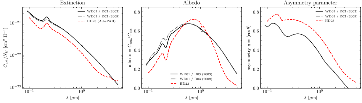
Figure 3: Extinction cross section per H (left), albedo (middle), and scattering-weighted asymmetry parameter (right) of the HD23 astroduct+PAH model (red dashed) overlaid on the WD01/Draine silicate+carbonaceous model in both the 2003 (black solid) and 2009 (gray dot-dashed) revisions, over the UV–NIR range.
