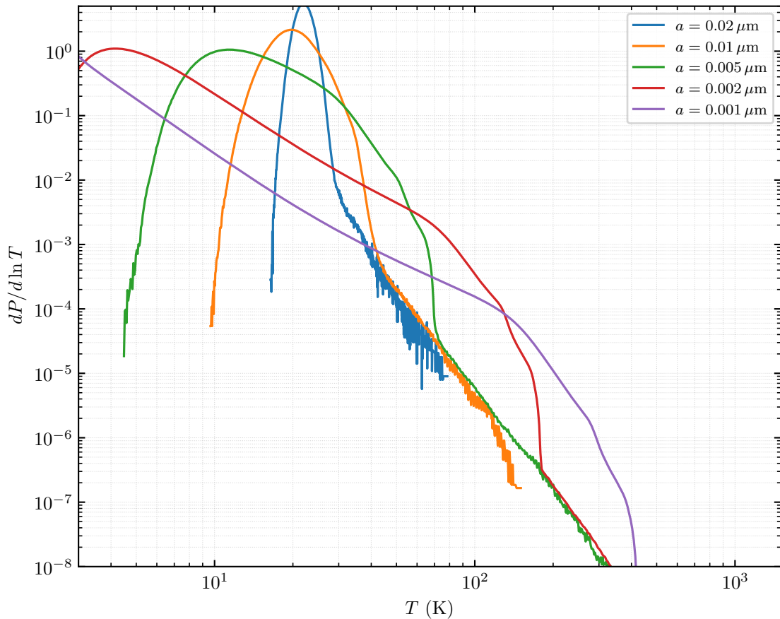
MC P(T) for graphite, Mathis ISRF ( U=1 )
