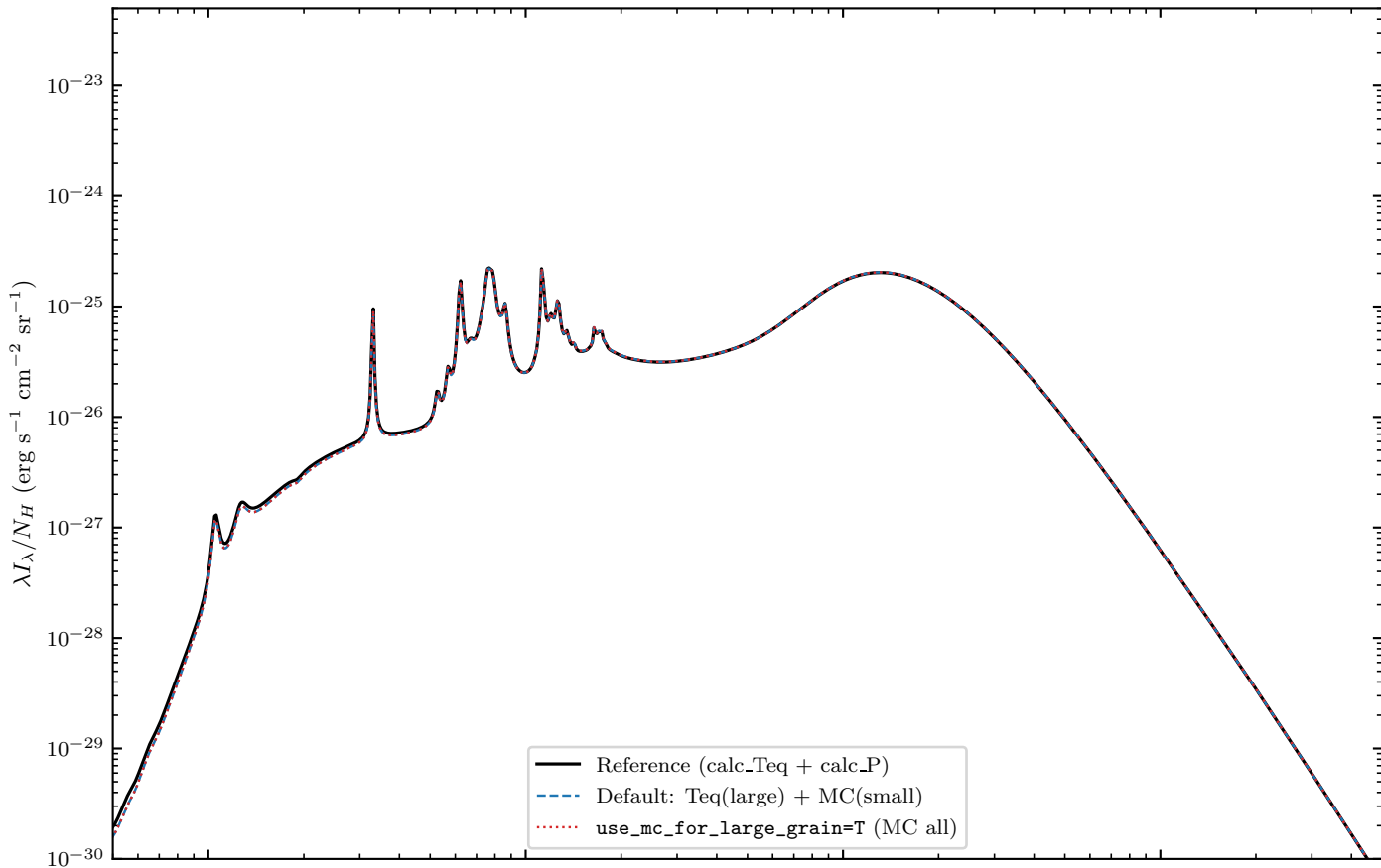
Two MC-pT solver modes vs production astrodust pipeline, \log U = 0.20 , Stage S2
