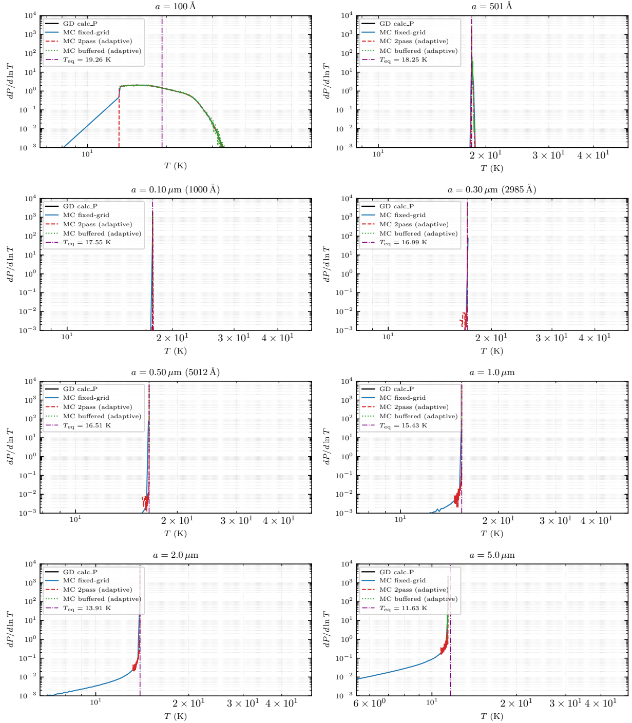
Figure 6: Single-grain dP/d \ln T for large astrodust grains ( a \in \{100, 501, 1000 \text{ \AA}, 0.3, 0.5, 1, 2, 5 \mu\text{m}\} , Stage 2 enthalpy, Mathis ISRF at \log U = 0.20 , N_{\text{e3t}} = 2 \times 10^5 ). Purple vertical line: T_{\text{eq}} from calc_Teq . Black: GD calc_P ; blue: fixed-grid MC; red dashed: 2pass adaptive; green dotted: buffered adaptive. With the adaptive \lambda_c(a) (§7.1) the MC trajectories hold tightly at T_{\text{eq}} for every panel from 100 \text{ \AA} to 5 \mu\text{m} ; the trajectory collapse toward CMB seen with a static \lambda_c = 1000 \mu\text{m} is fully removed.
