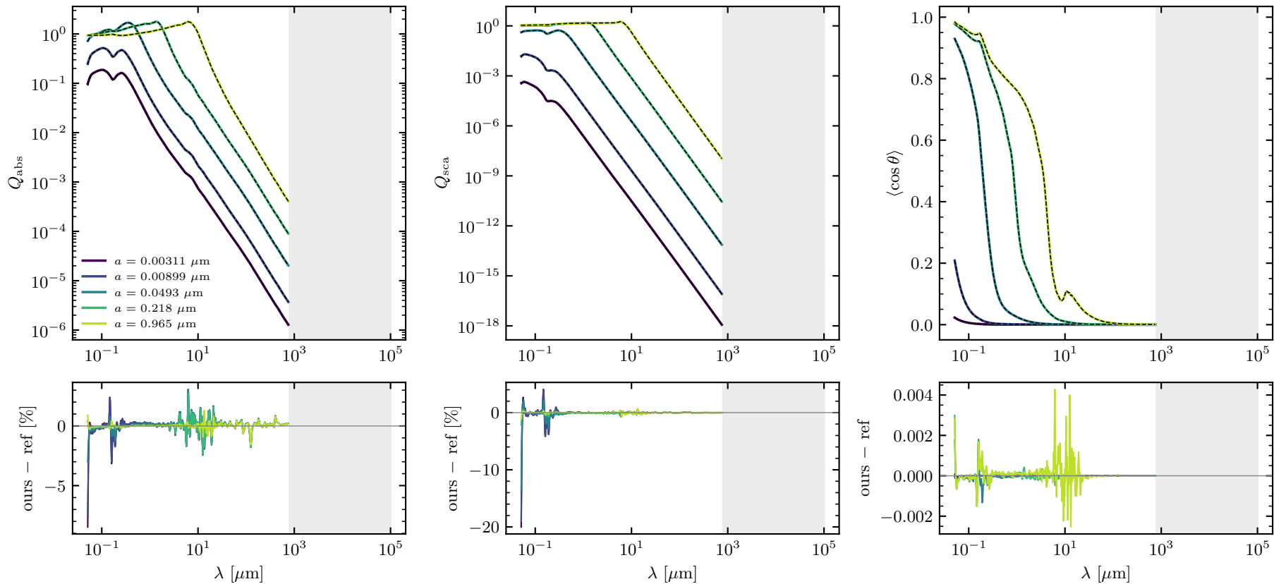
BE amorphous carbon spheres (Zubko et al. 1996) solid: DustEM Q_amCBEx / G_amCBEx, dashed: this work
