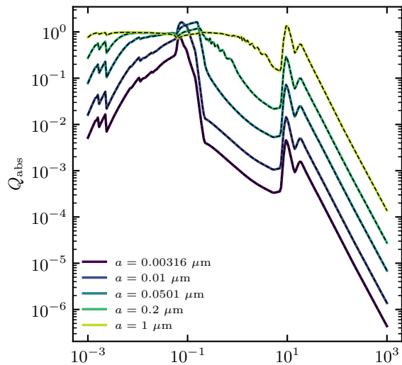
WD01 astrosilicate spheres solid: Draine suvSil_81, dashed: this work
