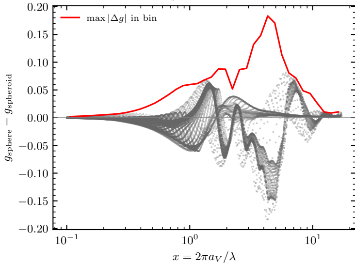
astrosilicate + 6% a-C, b/a = 0.4
