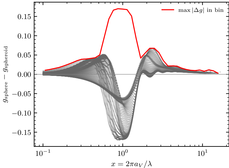
BE a-C, b/a = 1/3
