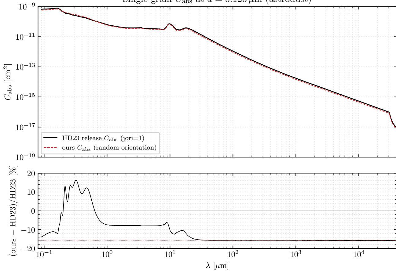
Single-grain C_{\text{abs}} at a = 0.126 \mu\text{m} (astrodust)
