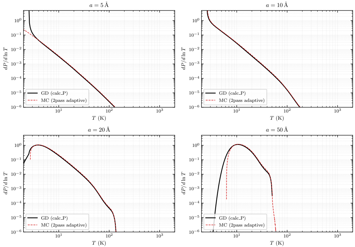
Figure 4: Single-grain dP/d \ln T for the astrodrust population (Stage 2 enthalpy), four selected radii in the stochastic regime ( a = 5, 10, 20, 50 \text{ \AA} ). Black: Guhathakurta–Draine matrix solver calc_P. Red dashed: Monte Carlo (mc_run_engine_2pass, adaptive histogram grid, N_{\text{evt}} = 5 \times 10^5 ). The two solvers overlap on the body and the high- T tail of each distribution; they differ only at the cold end, where the adaptive MC grid starts at the trajectory’s observed minimum temperature.
