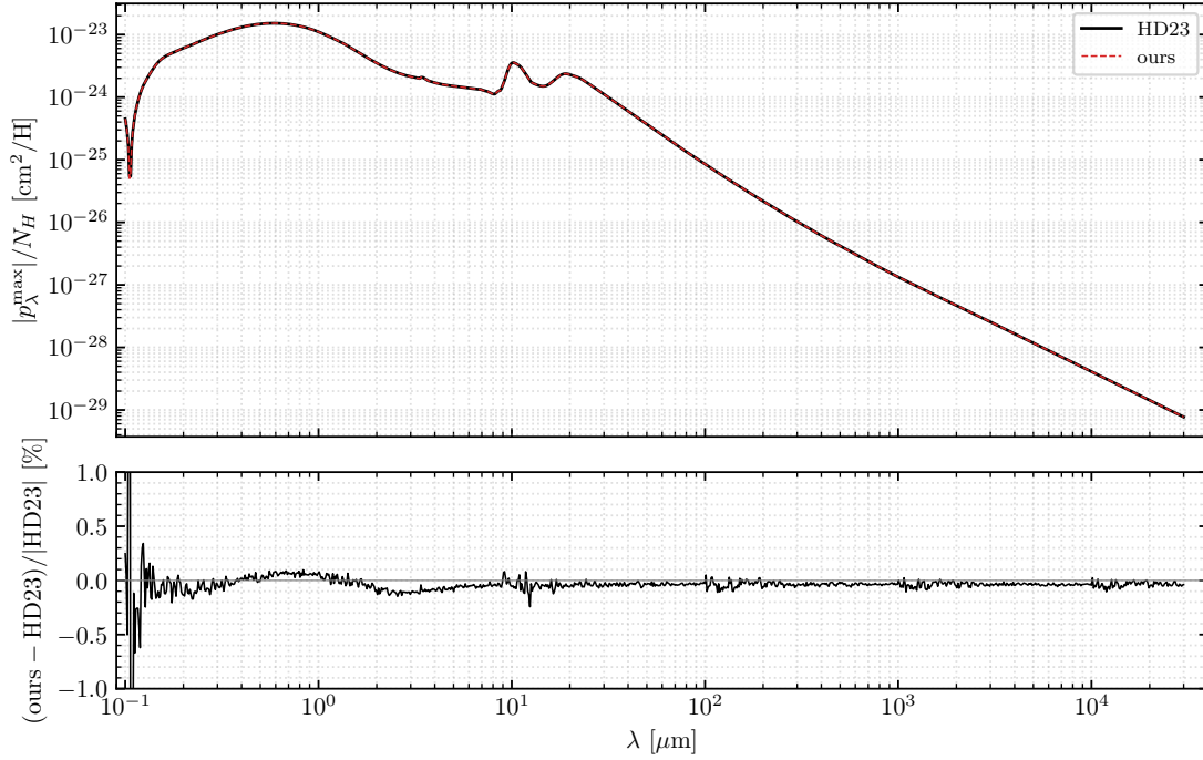
Figure 8: Top: |p^{\max}_{\lambda}|/N_H from HD23 polarized_extinction.dat (black solid) and from eq. 13 evaluated on the HD23 release Q tables (red dashed). Bottom: relative residual in percent. Peak value agrees to four significant figures.
