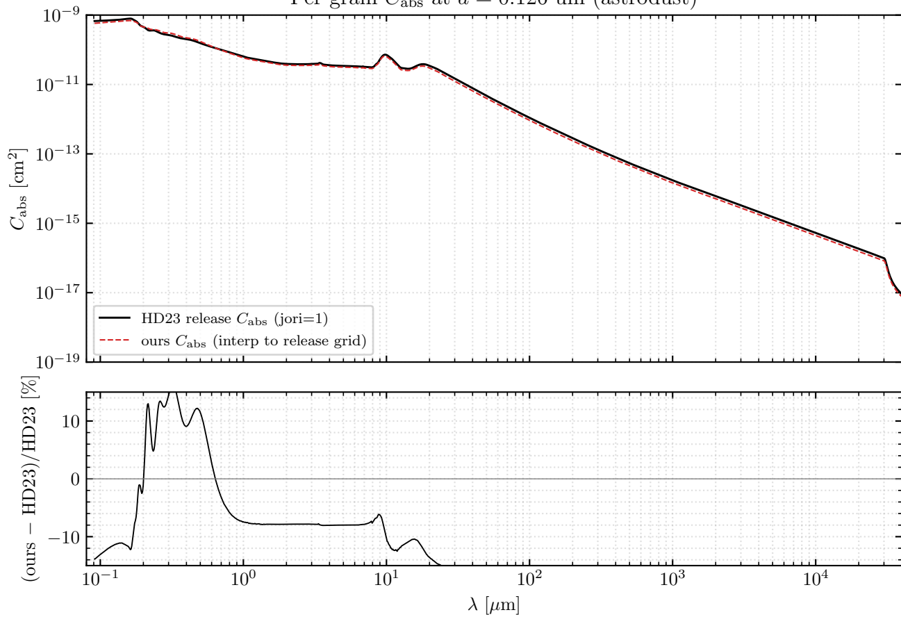
Per-grain C_{\text{abs}} at a = 0.126 \text{ } \mu\text{m} (astrodust)
