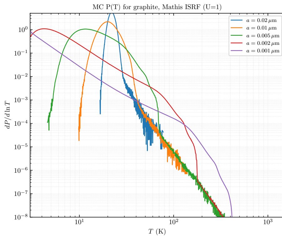
Figure 2: dP/d \ln T for graphite grains in the Mathis ISRF ( U = 1 ), for sizes a \in \{0.001, 0.002, 0.005, 0.01, 0.02\} \mu\text{m} . Compare with PIIM Figure 24.6.
