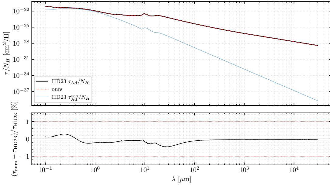
Figure 2: Top: HD23 \tau_{\text{Ad}}/N_H (black solid) and our value (red dashed), and HD23 \tau_{\text{Ad}}^{\text{sca}}/N_H (blue). Bottom: relative residual on \tau_{\text{Ad}}/N_H in percent. The acceptance band ( \pm 1\% ) is shown in dotted red.
