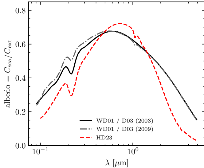
Albedo
