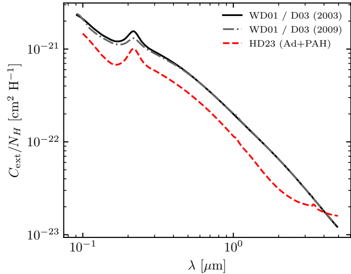
Extinction
