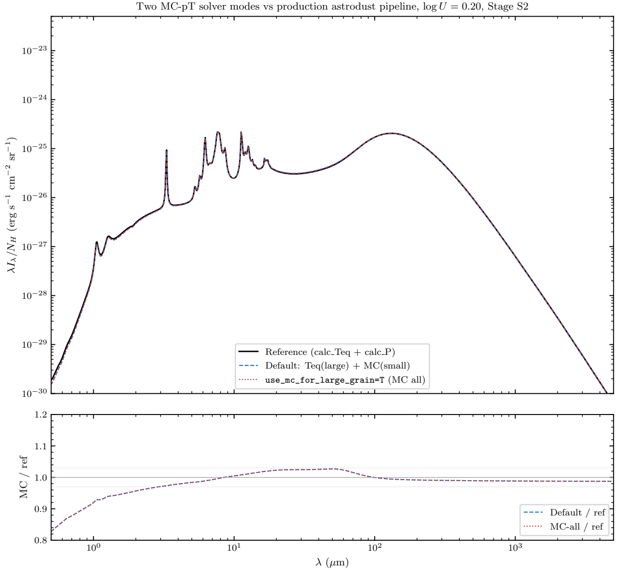
Figure 3: Two MC-pT solver modes versus the production astrodrust pipeline, for the HD23 astrodrust+PAH model in the Mathis ISRF at \log U = 0.20 , Stage 2 enthalpy. Both modes use the adaptive 2pass histogram engine, the integrator step cap (§2.), the single-grain energy-conservation rescale and charge-resolved PAH (§5.2), and the adaptive Draine & Anderson (1985) cutoff \lambda_c(a) = hc/(\delta T_{\text{thresh}} T_{\text{eq}} C(T_{\text{eq}})) with \delta T_{\text{thresh}} = 0.01 (§7.1). Top: \lambda I_\lambda / N_H . Bottom: ratio of each mode to the reference (note the expanded 0.8–1.2 vertical scale). The default mode (blue dashed) and the all-MC mode (red dotted) are indistinguishable and both match the reference to within 1–3% in every band (NIR 0.97, MIR 1.01, FIR 1.00, sub-mm 0.99); the dip below 1 \mu\text{m} is at the optical/far-NIR edge, \sim 5 decades below the peak and carrying negligible power. The \sim 30\% all-MC FIR underprediction of earlier versions — from large-grain trajectory collapse under a static \lambda_c = 1000 \mu\text{m} and from hot-tail over-population by the uncapped integrator — is fully removed.
