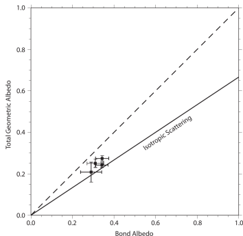
Figure 10: Total (wavelength-integrated) geometric albedo versus Bond albedo for a Lambert sphere (solid, A_g/A_B = 2/3 ) and for Uranus, Neptune, Saturn, Jupiter (points, in order of increasing A_B ). The dashed line is A_g = A_B . Adapted from Rowe et al. (2006); reproduced from Seager (2010), Fig. 3.7.
