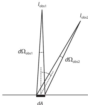
Figure 14: Intensity observed by a distant viewer. The solid angle subtended by dA is smaller at observer 2 than at observer 1. Reproduced from Seager (2010), Fig. 2.8.
