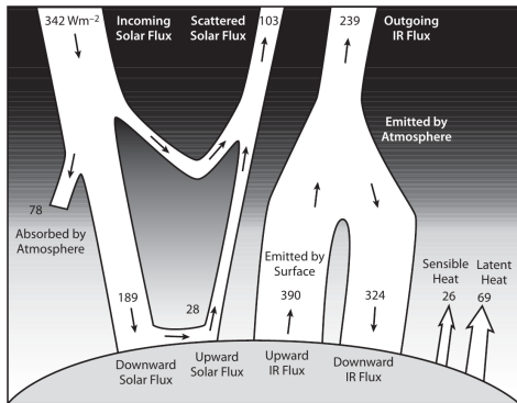
Figure 2: Energy balance of Earth's atmosphere (global means, in \text{W m}^{-2} ). Seager (2010), Fig. 6.1.
