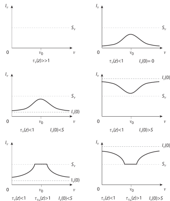
Figure 10: Line formation for a source function constant with depth and frequency. Seager (2010), Fig. 6.9, after Rutten.
