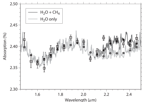
Figure 8: HST/NICMOS transmission spectrophotometry of HD 189733b (squares) with models containing H 2 O only (gray) or H 2 O + CH 4 (black). Seager (2010), Fig. 6.7.
