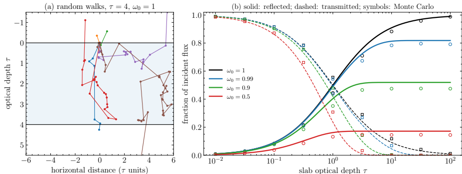
Figure 14: A homogeneous slab with isotropic scattering, lit from above by diffuse light, no emission. Lines: two-stream (hemispheric closure); symbols: Monte Carlo. Script scripts/make_twostream_slab.py .
