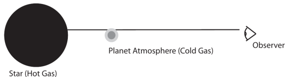
Figure 5: Origin of a transit transmission spectrum: hot stellar light through the cool planetary atmosphere. Seager (2010), Fig. 6.5.
