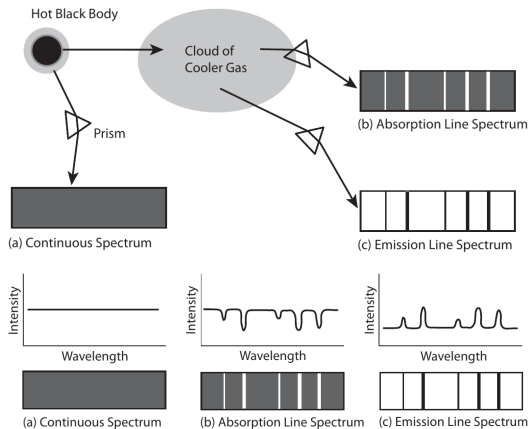
Figure 3: Origin of the three kinds of spectra (top) and what they look like over a narrow wavelength range (bottom). Seager (2010), Figs. 6.2 and 6.3.
