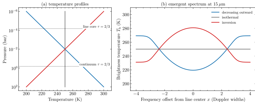
Figure 6: A line with a Gaussian opacity profile (peak 10^4 times the continuum) in three LTE atmospheres. Left: the temperature profiles and the pressures where \tau = 2/3 in the continuum and at line center. Right: the emergent flux as a brightness temperature. Computed with F = 2\pi \int B E_2(\tau_\nu) d\tau_\nu ; script scripts/make_line_formation.py .
