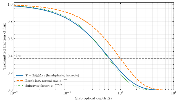
Figure 1: Hemispheric transmission \mathcal{T} = 2E_3(\Delta\tau) of an isothermal slab compared with Beer's law for a normal ray and with the diffusivity-factor approximation e^{-5\Delta\tau/3} .
