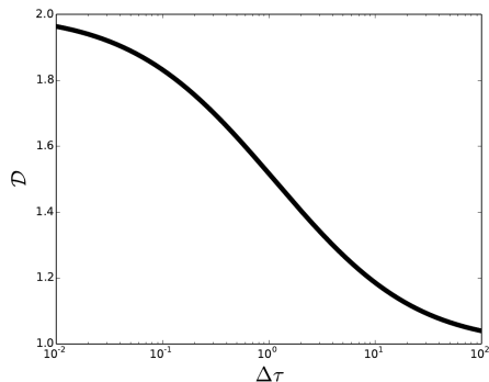
Figure 13: The diffusivity factor that makes the two-stream transmission exact for a purely absorbing isothermal layer. Heng (2017), Fig. 3.1.
