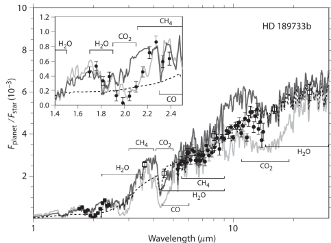
Figure 9: Secondary-eclipse data for HD 189733b: Spitzer photometry (squares), Spitzer/IRS (circles), HST/NICMOS (inset), with best-fit models. Seager (2010), Fig. 6.8.
