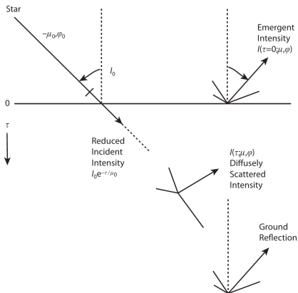
Figure 11: The attenuated direct beam from the star and the diffusely scattered intensity. Seager (2010), Fig. 6.10, after Chamberlain & Hunten.
