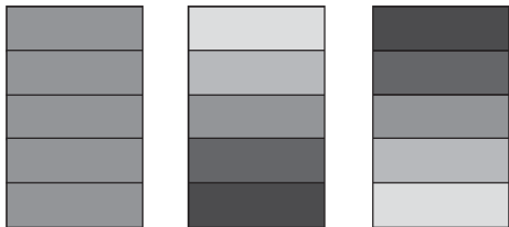
Figure 4: A five-layer atmosphere; darker means hotter. Left: isothermal. Middle: hot at depth, cooler above. Right: a temperature inversion. Seager (2010), Fig. 6.4.
