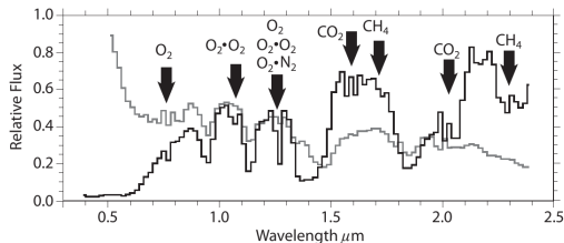
Figure 12: Earth as an exoplanet: hemispherically integrated scattered light from earthshine (gray) and the transmission spectrum measured during a lunar eclipse (black). Seager (2010), Fig. 6.11, from Pallé et al. (2009).
