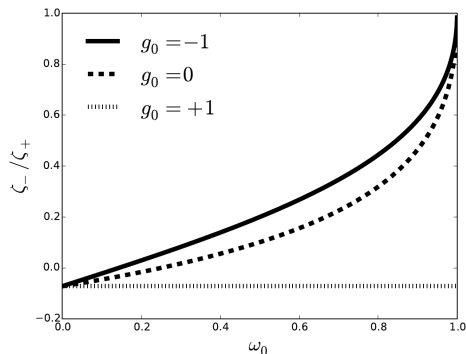
Figure 15: Spurious enhancement or reduction factor \zeta_-/\zeta_+ of the Eddington closure for an opaque layer. Heng (2017), Fig. 3.2.
