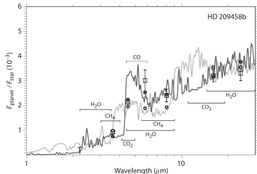
Figure 7: HD 209458b, Spitzer secondary-eclipse photometry (squares) with a model with absorption features only (gray) and one with a deep inversion (black). Seager (2010), Fig. 6.6.
