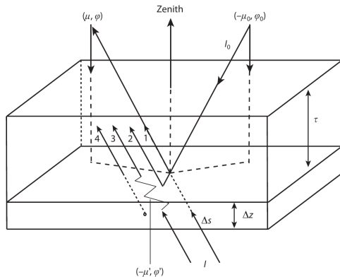
Figure 16: The four processes that change the intensity in a volume element: (1) attenuated starlight, (2) singly scattered starlight, (3) diffusely scattered radiation, (4) thermal emission. Seager (2010), Fig. 6.12, after Liou.
