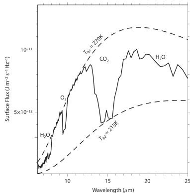
Figure 7: Earth's mid-infrared spectrum: T_b(12\text{ }\mu\text{m}) \simeq 270\text{ K} but T_b(14.2\text{ }\mu\text{m}) \simeq 215\text{ K} . Reproduced from Seager (2010), Fig. 3.4.
