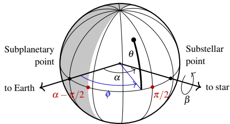
Figure 9: Coordinates for the phase-dependent scattered flux. \theta is latitude from the intensity equator, \phi longitude from the sub-Earth point, \alpha the phase angle, \beta the azimuth of the observer about the star direction (next slide). After Sobolev (1975); redrawn after Seager (2010), Fig. 3.6.
