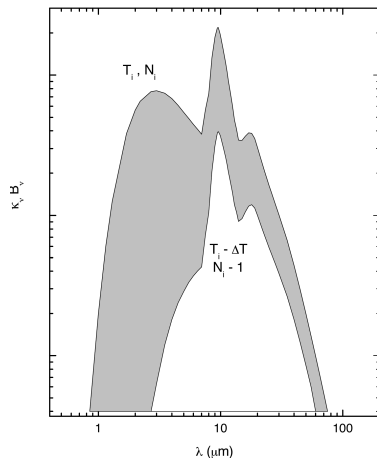
Fig. 1 of Bjorkman & Wood (2001): dust emissivity \kappa_v B_v(T) before (lower) and after (upper) one absorption; the reemitted packet samples the shaded area.
