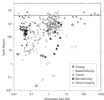
Figure 4: Known exoplanets as of January 2010, by discovery technique; circled points have an atmosphere measurement; Solar System planets by initial; the line is 13 M_J . Seager (2010), Fig. 1.5.
