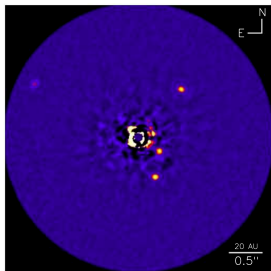
Figure 3: The four young gas-giant planets of HR 8799 (Marois et al. 2008, 2010), starlight suppressed. Heng (2017), Fig. 1.5.
