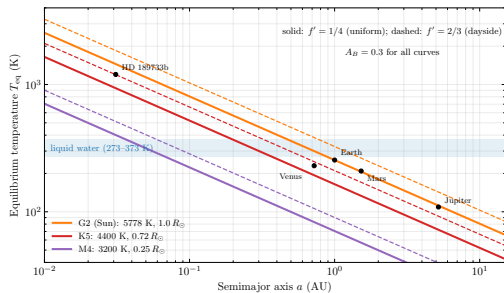
Figure 4: Equilibrium temperature versus semimajor axis for three host stars, with A_B = 0.3 ; solid f' = 1/4 , dashed f' = 2/3 . Points are Solar System T_{\text{eq}} values (Table 3.1) and HD 189733b.
