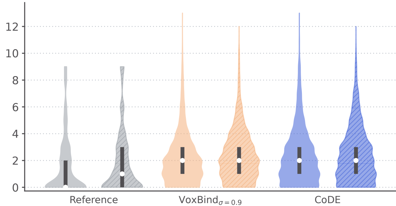
Hydrophobic contacts
