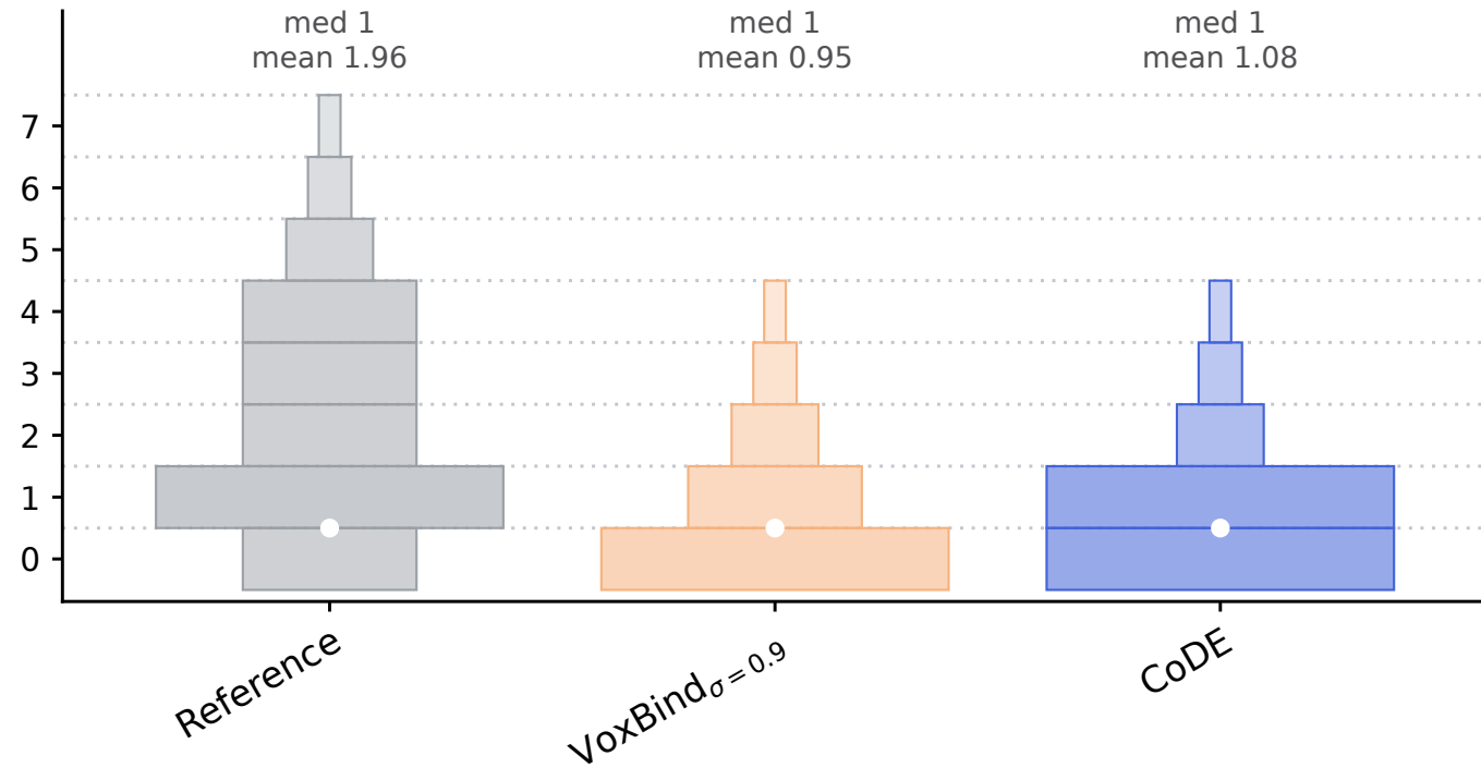
H-bonds acceptor
