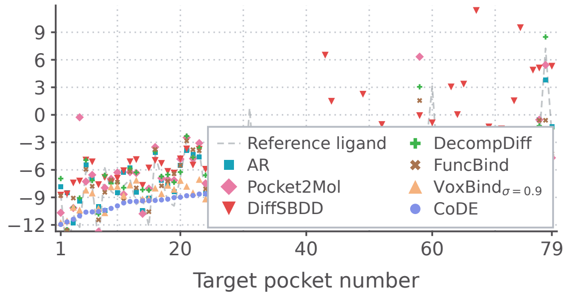
Vina Score mean
