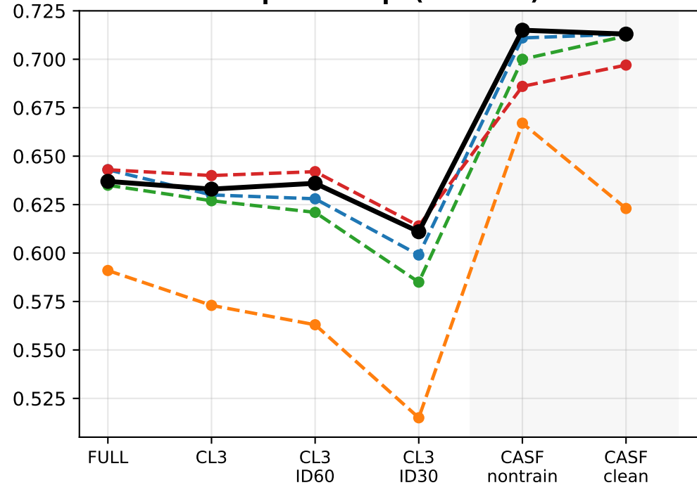
Spearman \rho ( \uparrow better)
