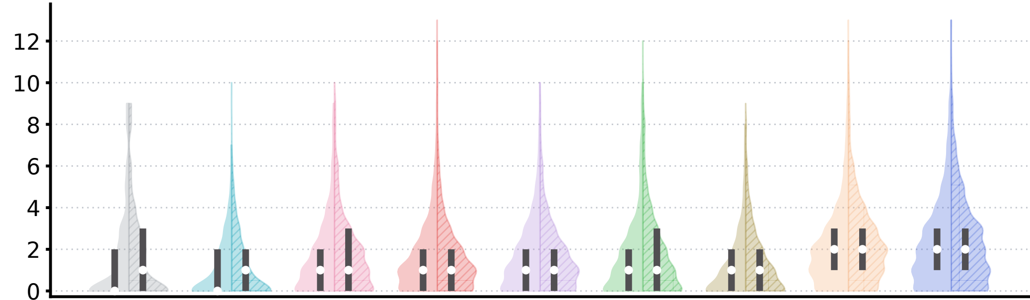
Hydrophobic contacts
