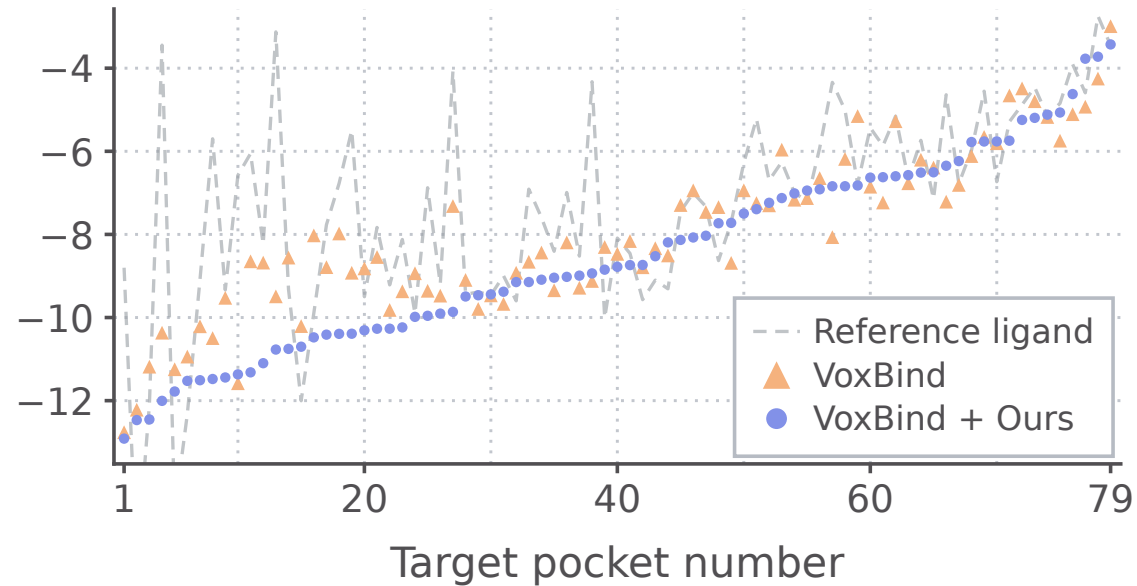
Vina Dock mean
