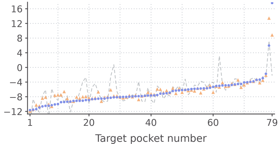
Vina Score median
