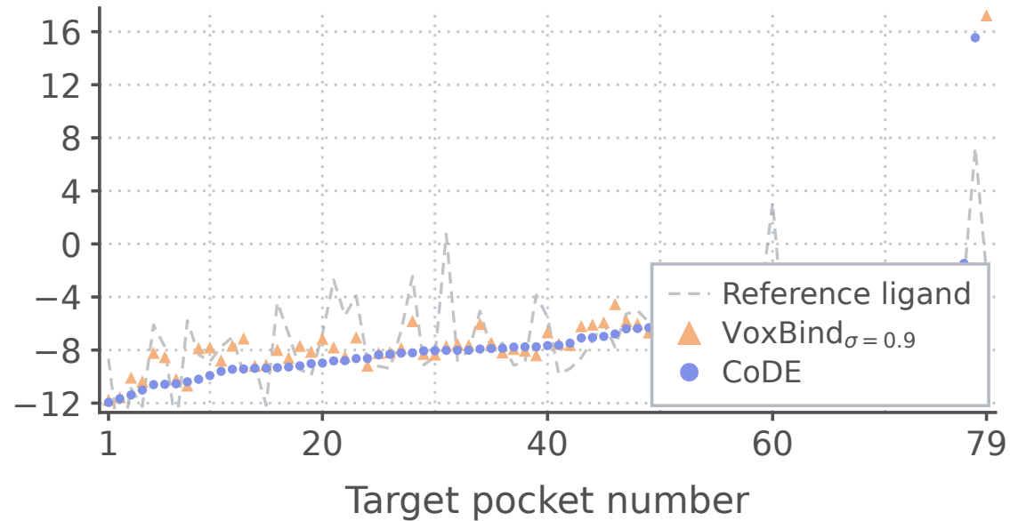
Vina Score mean
