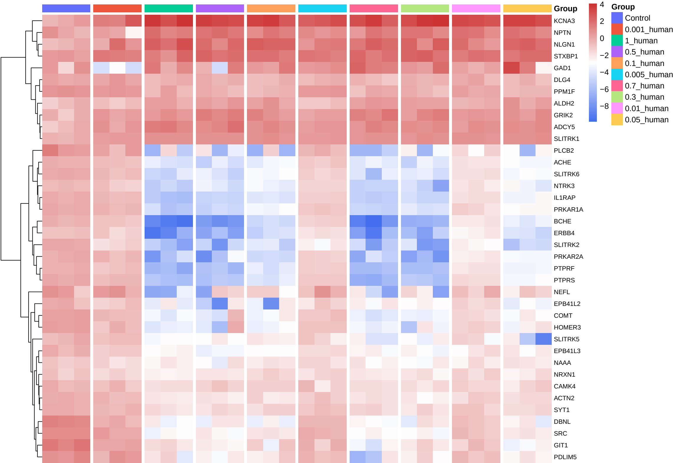
38 DEPs: Neuronal System
