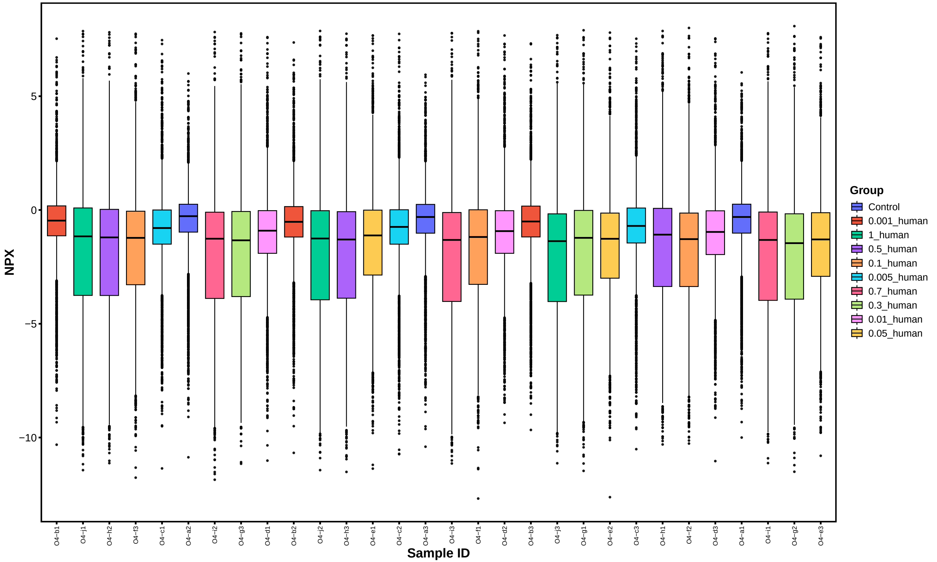
NPX Distribution by Sample
