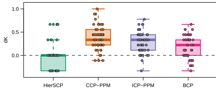
Signed segment-count error ( K_{\text{hat}} - K )
