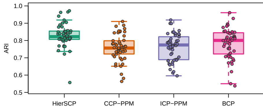
Adjusted Rand Index
