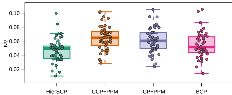
Normalized variation of information (lower = better)
