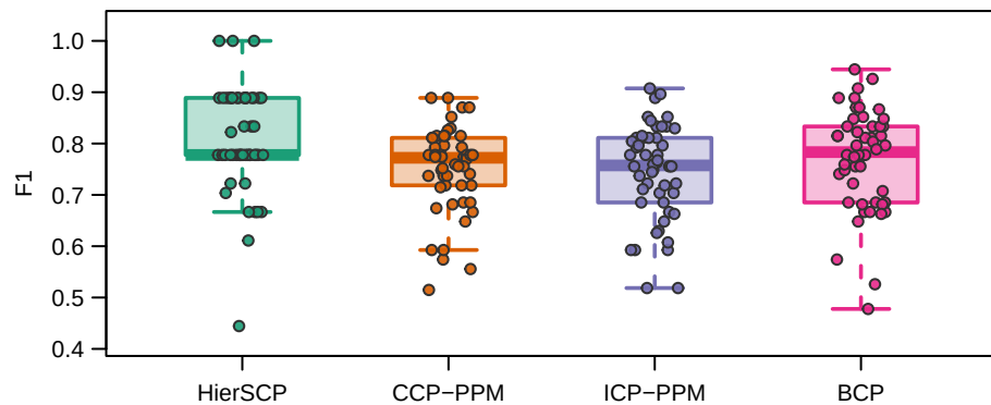
F1 score (margin = 10 timepoints)
