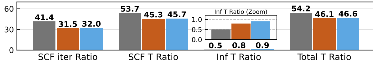
QH9-dynamic (300k-geo)
