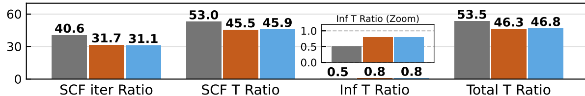
QH9-stable (id)
