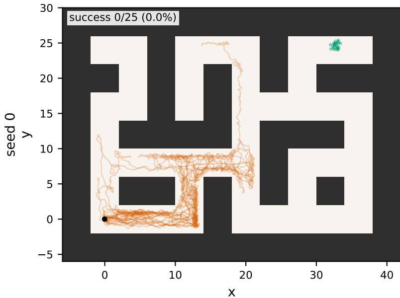
Shared actor
