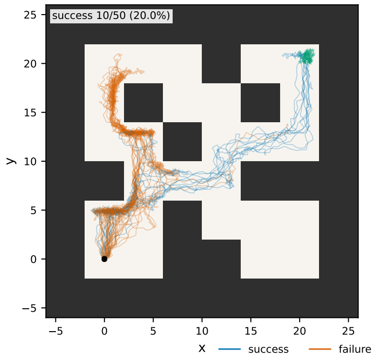
(a) Shared actor
