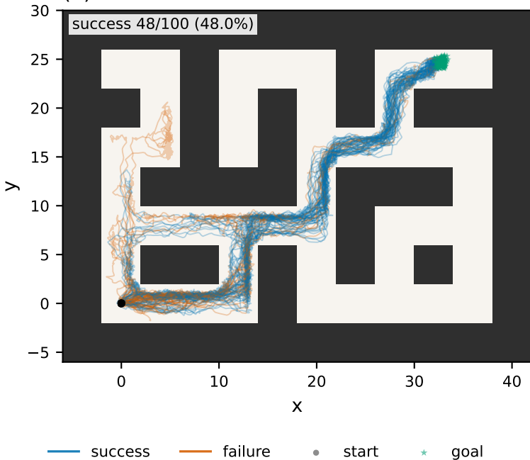
(a) TD3+RAPO
