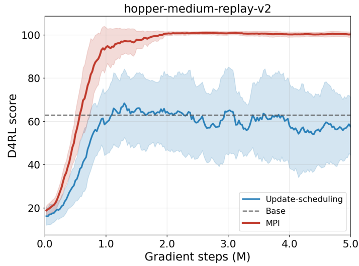
Figure 1: TD3+BC: MPI vs. actor-update scheduling on hopper-medium-replay-v2 . Base is original TD3+BC; Actor-update scheduling uses five TD3+BC actor updates per delayed actor slot; MPI uses one base update plus four re-centered refinements ( K = 4 ). All runs use the original TD3+BC configuration; shaded regions denote standard deviation over 4 seeds.
