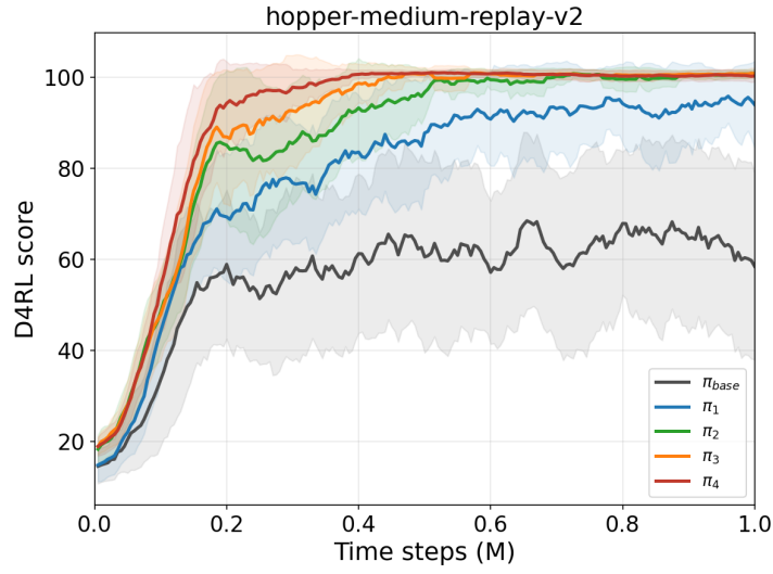
Figure 1: TD3+BC: Actor-wise diagnostic training curves on hopper-medium-replay-v2 under the TD3+BC-matched setup. It compares \pi_{base} and recentered actors \pi_1 - \pi_4 to isolate the effect of recentering. All runs use the original TD3+BC configuration; shaded regions denote standard deviation over 4 seeds.
