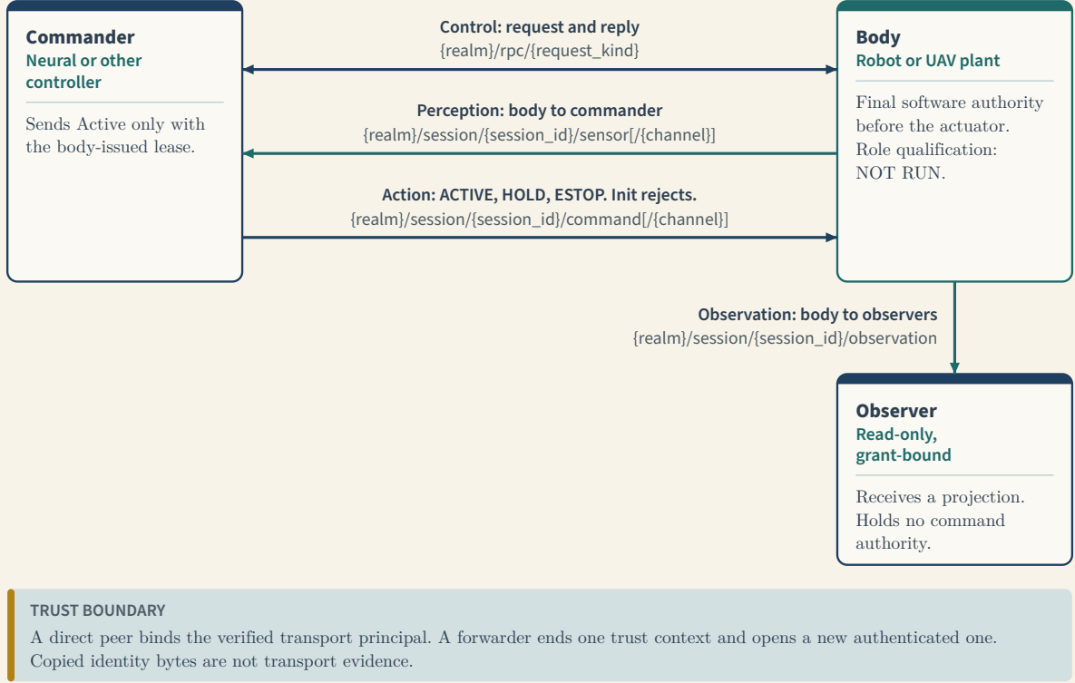
Figure 5: Topology. The routes are the current wire 1.0 key grammar. The body is the final software authority before the actuator.
