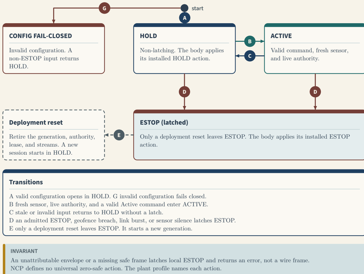
Figure 15: Current plant-admission states of the compatibility governor.
