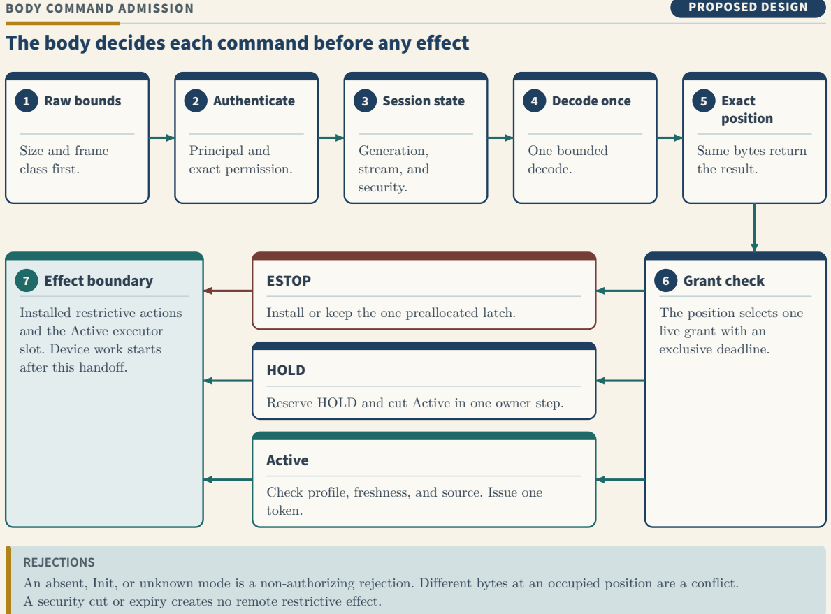
Figure 11: Body command admission. ESTOP, HOLD, and Active follow different paths to the effect boundary.
