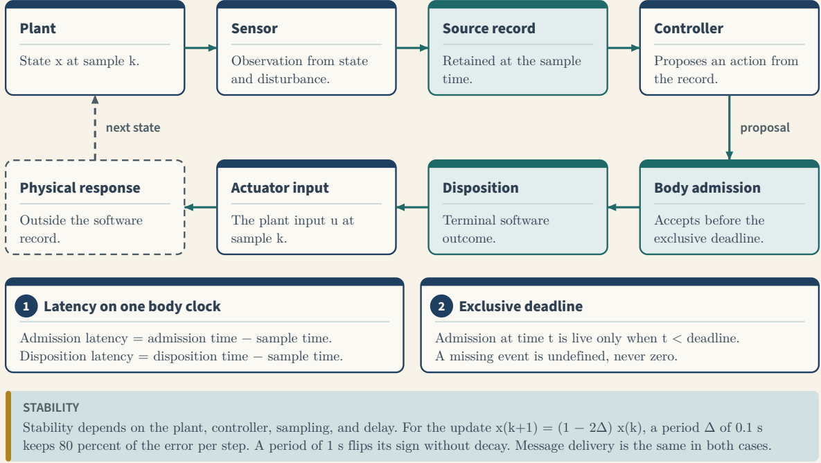
Figure 12: One feedback cycle. NCP records three software events. It cannot measure the physical response.
