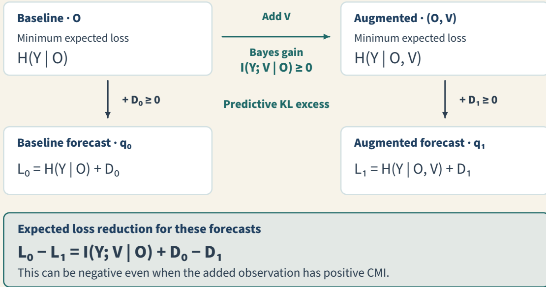
Figure 1: Conceptual fixed-law expected-loss identity: the augmented observation lowers unrestricted Bayes loss by conditional information, while predictive KL excess determines the loss of supplied forecasts.
