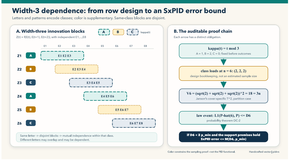
Figure 1: A width-three construction and the five logically distinct obligations in the proof. The letters A, B, and C and their long-dash, dotted, and compound-dash outlines carry the class encoding; color is supplementary. Same-class innovation blocks are disjoint, whereas blocks in different classes may overlap. The right panel separates design bookkeeping, the probability theorem, and the deterministic SxPID transfer.
