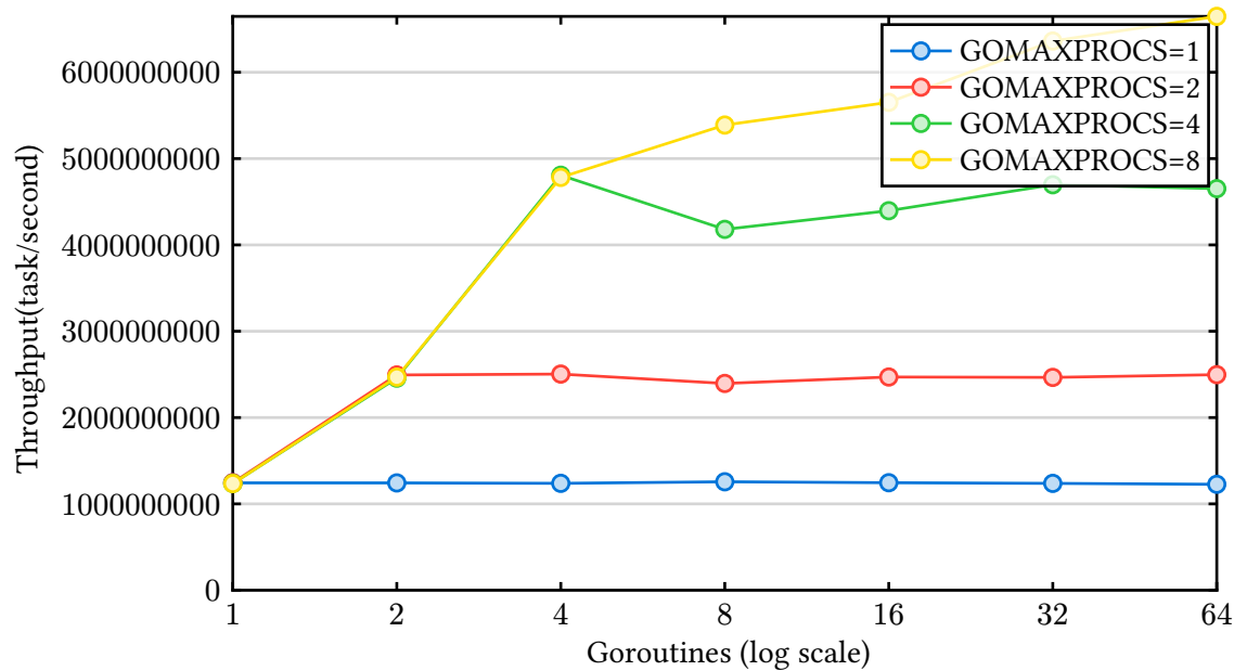
Figure 1: CPU-bound Throughput Comparison
