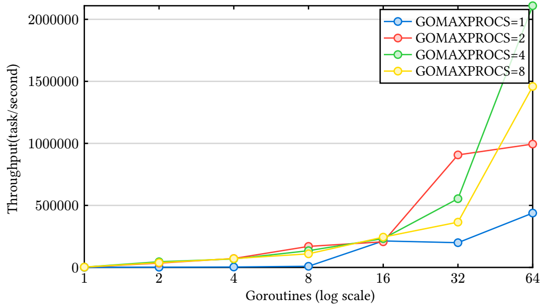
Figure 7: Sleep-bound Throughput Comparison
