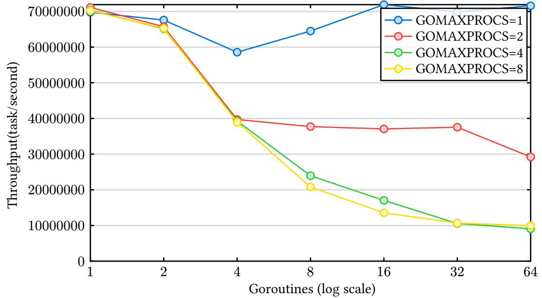
Figure 4: Mutex-bound Throughput Comparison
