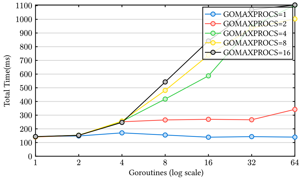
Figure 6: Mutex-bound Throughput Comparison
