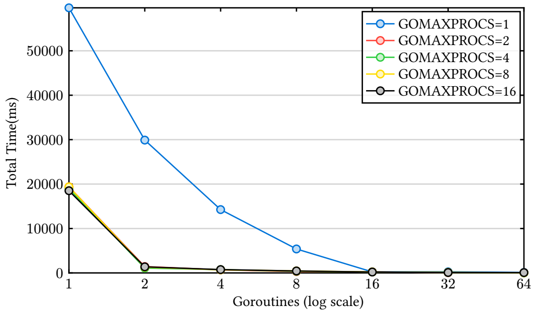
Figure 9: Sleep-bound Throughput Comparison
