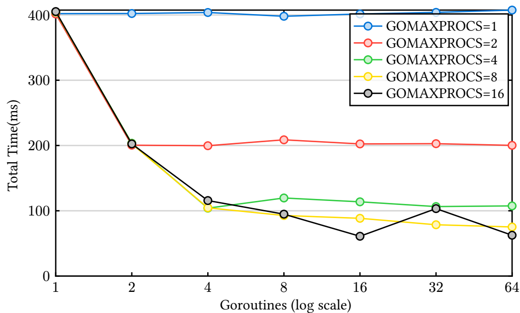
Figure 2: CPU-bound Throughput Comparison
