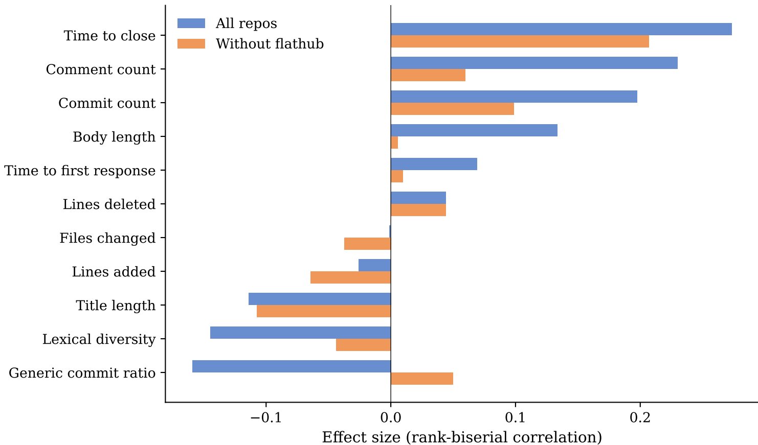
PR-level effect sizes: with vs. without flathub
