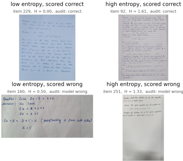
Figure 2. Four perception cases. Self-disagreement helps when wrong answers produce varied samples, but it is weakest when the samples mostly agree on the same wrong reading. The top panels were scored correct and the bottom panels were scored wrong; the left panels have low entropy and the right panels have high entropy. Each panel gives its item, entropy and human-audit verdict.
