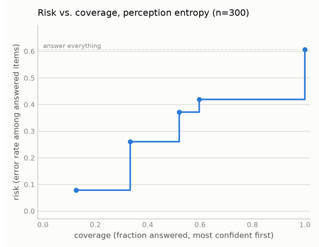
Figure 1. Risk–coverage against the frozen transcription scorer for perception entropy, Qwen2.5-VL-3B, n = 300 . Deferring the highest-entropy items first traces AURC 0.410 against a 0.607 random-deferral baseline. The curve is the practitioner-facing form of the result: at a 10% risk target the rule retains 21.3% coverage, and token log-probability cannot hold error below 40% at any coverage.
